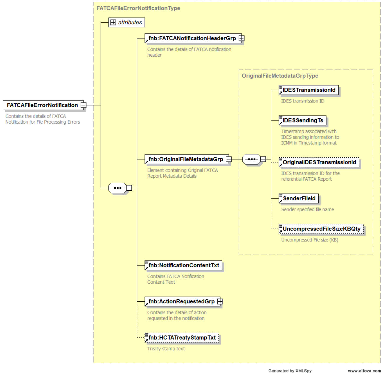
Figure 4: OriginalFileMetadatGrp Type Layout
